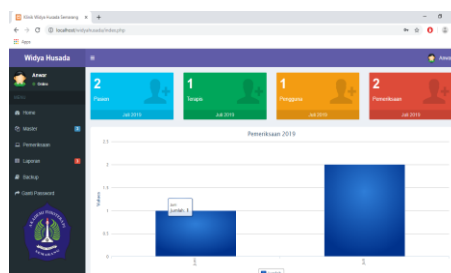
Gambar 5 Halaman Home
