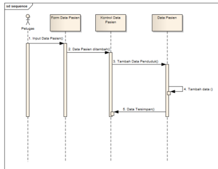
Gambar 3 Sequence Diagram
