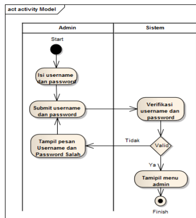
Gambar 2 Activity Diagram
