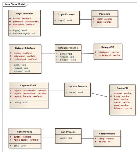
Gambar 4 Class Diagram
