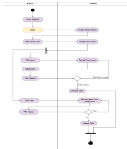
Gambar 9. Activity Diagram Kelola User
