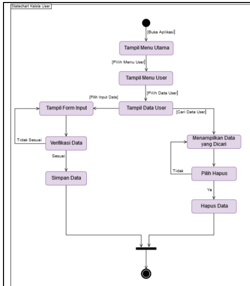
Gambar 4. Statechart Diagram Kelola User
