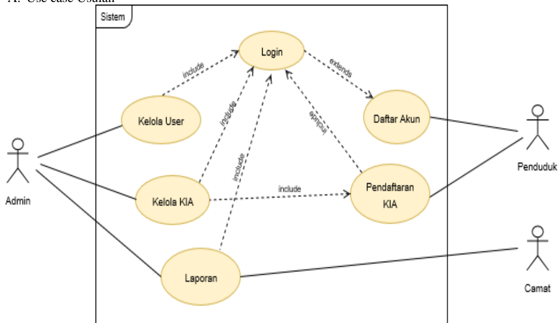
Gambar 3. Use Case Diagram Usulan
