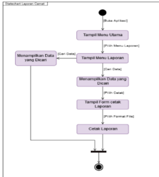
Gambar 8.Statechart Diagram Laporan Camat
