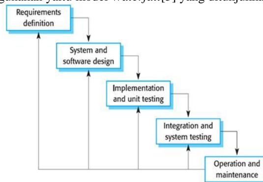
Gambar 1. Metode Waterfall
