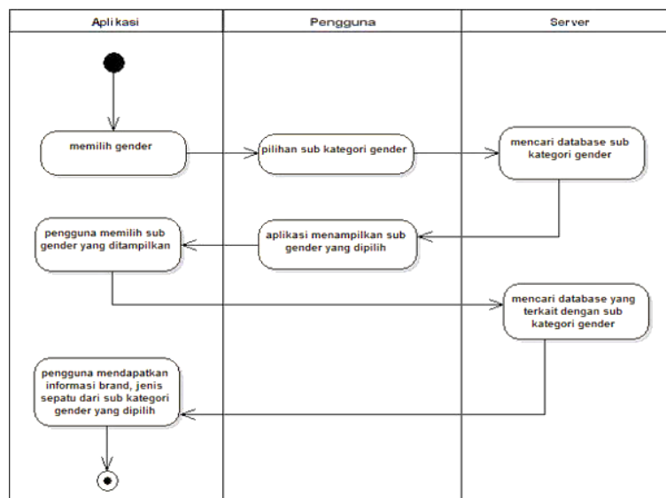
Gambar 4. Activity Diagram Gender
