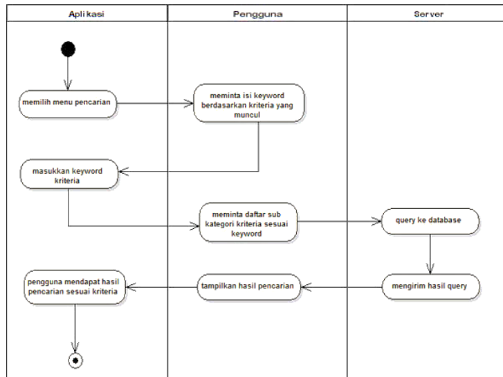
Gambar 5. Activity Diagram Pencarian Kriteria
