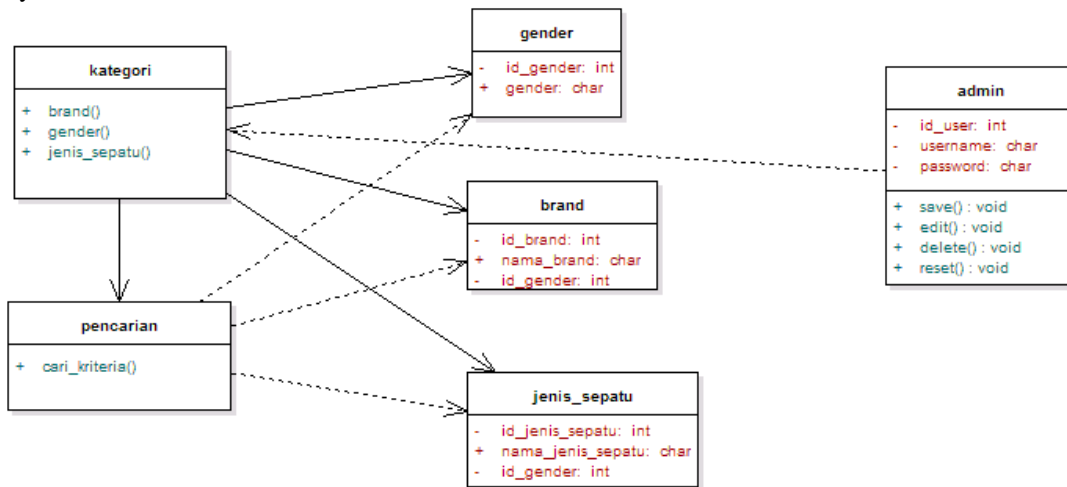
Gambar6 : Diagram Class
