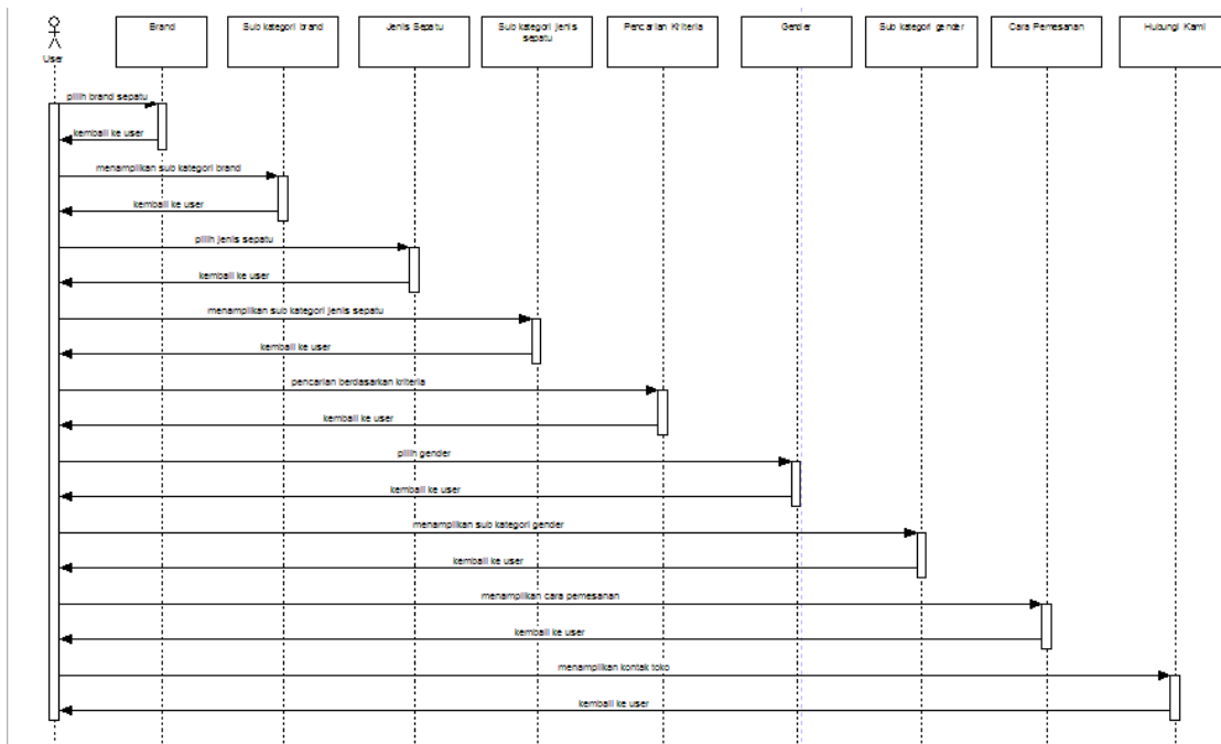
Gambar 7 : Diagram Sequence
