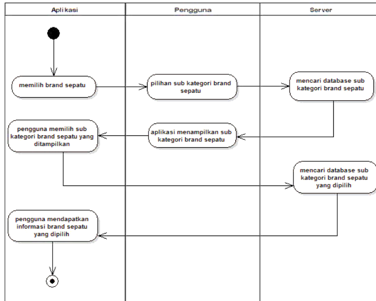
Gambar 2. Activity Diagram Brand
