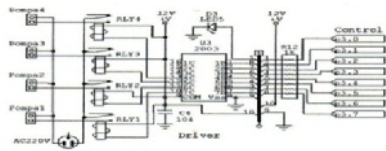
Gambar 9 Rangkaian Driver Relay
