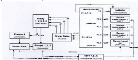
Gambar 3.5 Blok Diagram Automatic Watering Plant
