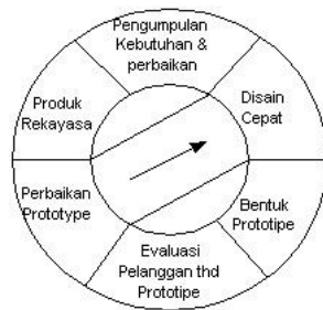
Gambar 4.1 . Prototyping Method
