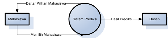
Gambar 1. Context Diagram
