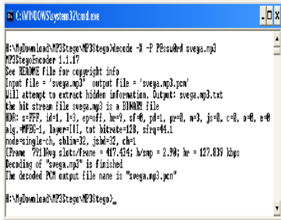
Gambar 5. Proses Decode
