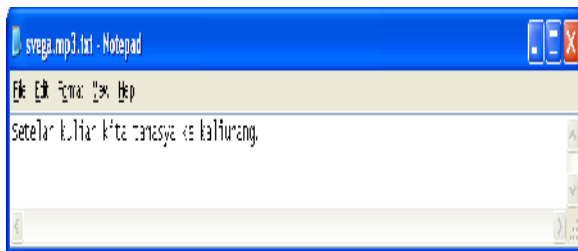
Gambar 6. Hasil Decode
