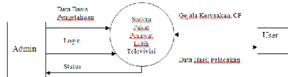
Gambar 1. DFD Level 0
